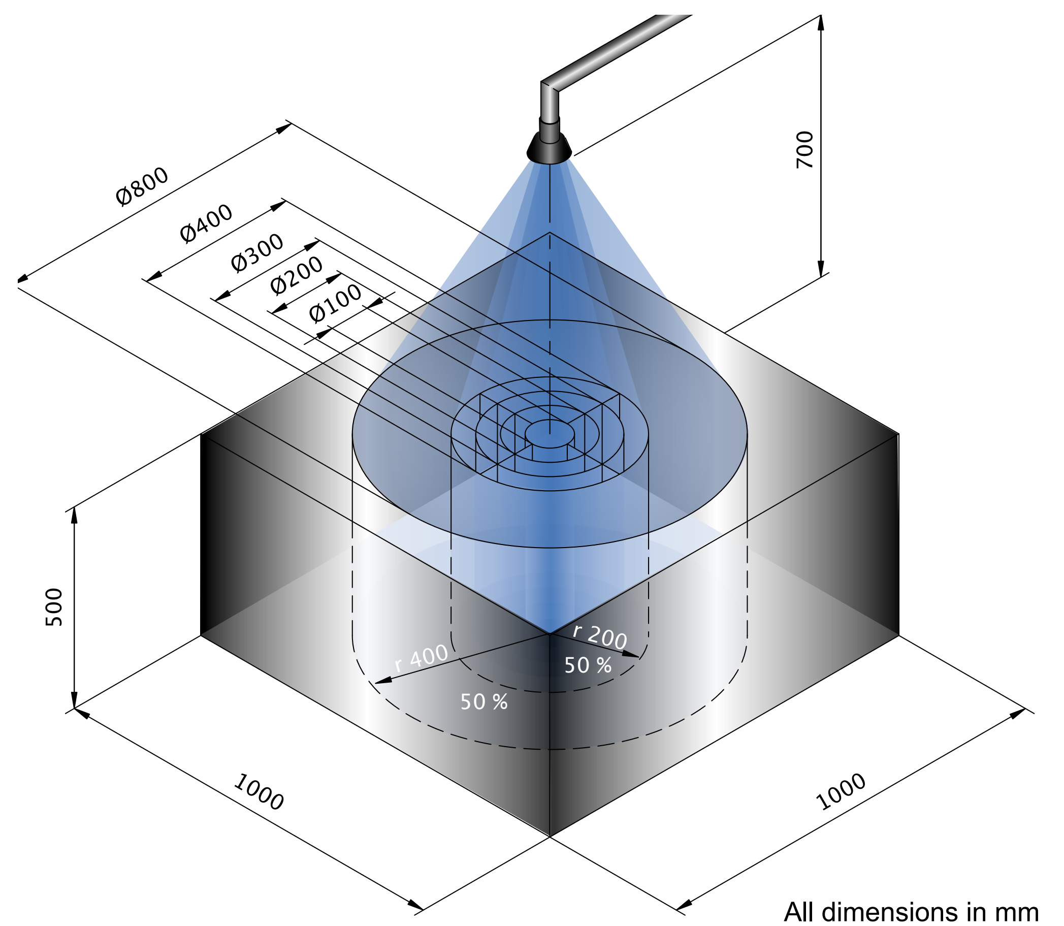
FIGURE 1 - TYPE TESTING OF WATER DISTRIBUTION
